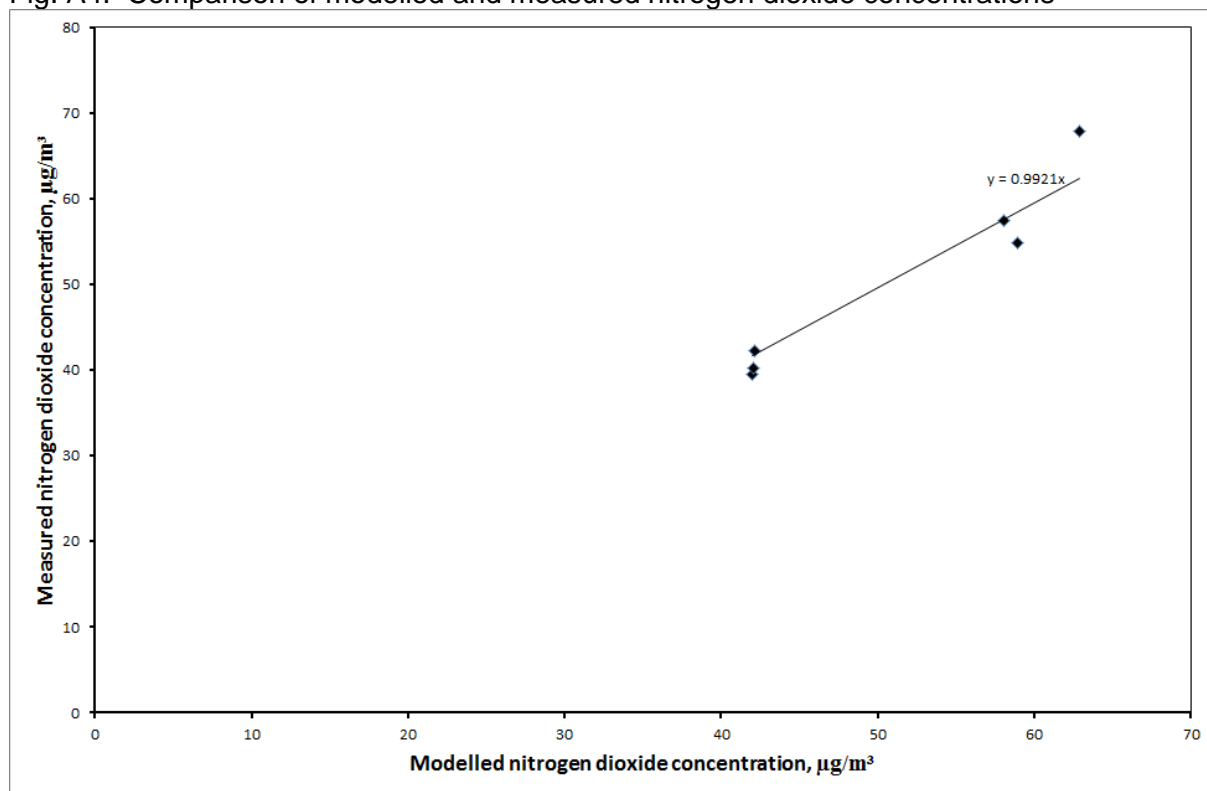
Fig. A4: Comparison of modelled and measured nitrogen dioxide concentrations
