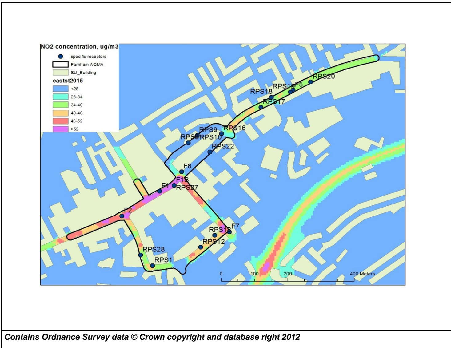
Fig. A2: Modelled nitrogen dioxide concentrations, 2015 with development
