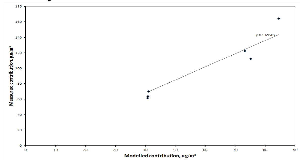
Fig. A3: Comparison of unadjusted modelled and measured road contributions to oxide of nitrogen concentrations
