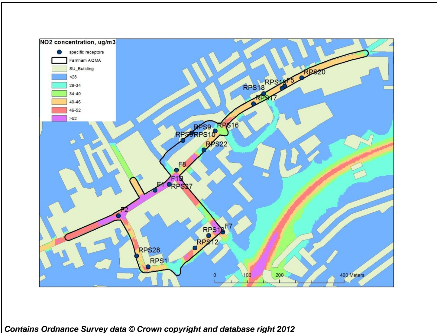
Fig. A1: Modelled nitrogen dioxide concentrations, 2010
